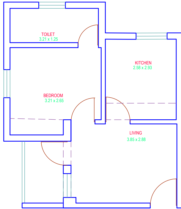
PROPOSED CIVIL CHANGE PLAN
