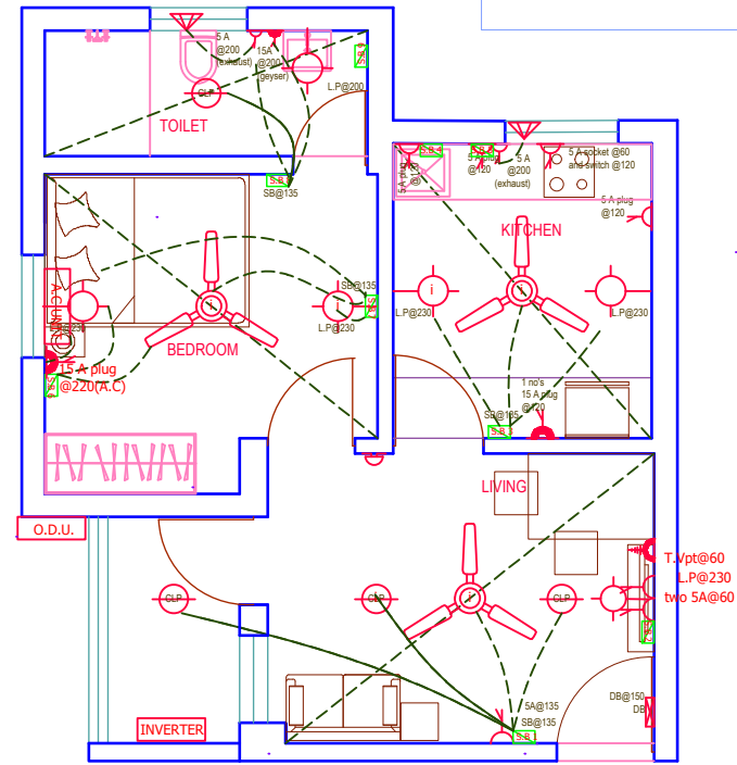
PROPOSED ELECTRICAL PLAN
