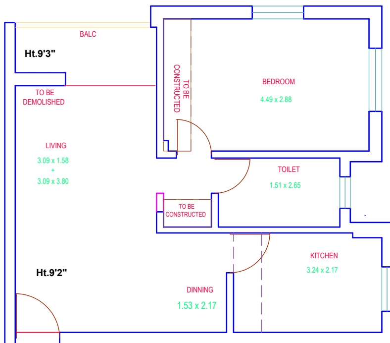
PROPOSED CIVIL CHANGE PLAN
