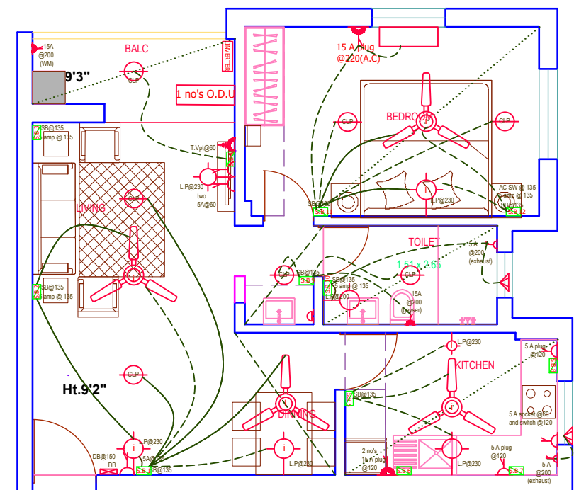
PROPOSED ELECTRICAL PLAN
