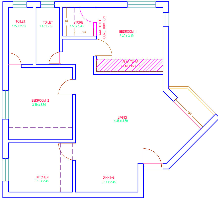
PROPOSED CIVIL CHANGE PLAN
