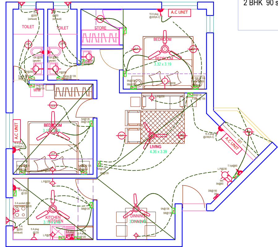
PROPOSED ELECTRICAL PLAN
